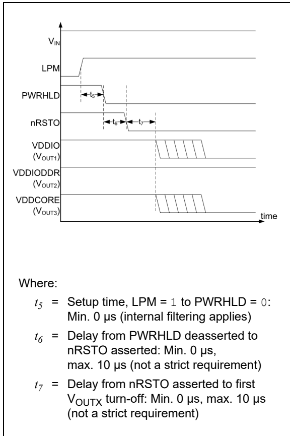
FIGURE 4-8: Entering Hiberate Mode Timing Diagram.
