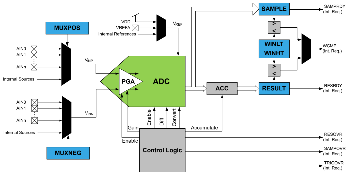
Figure 31-1. Block Diagram
