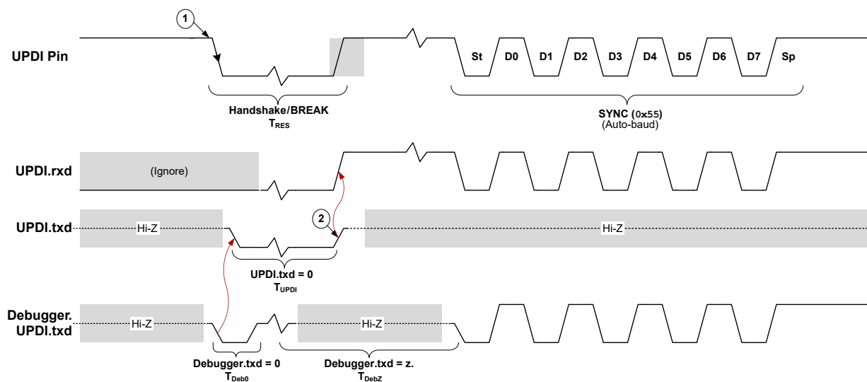
① Drive low from the debugger to request the UPDI clock. ② UPDI clock ready; Communication channel ready.
