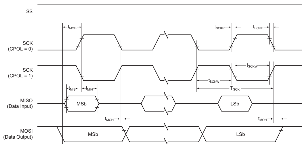
Figure 35-4. SPI - Timing Requirements in Host Mode
