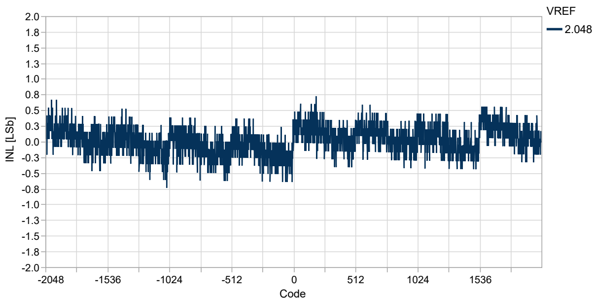
Figure 34-58. INL vs. Code ( V_{DD} = 5.0\text{V} , T = 25^{\circ}\text{C} , f_{ADC} = 145 ksp/s), Differential, External 2.048V Reference
