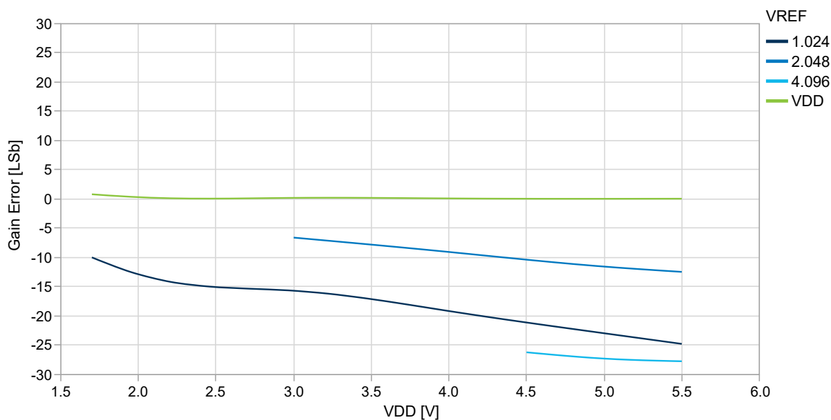
Figure 34-57. Gain Error vs. V_{DD} ( f_{ADC} = 145 ksp/s) at T = 25^{\circ}\text{C} , Differential, REFSEL = Internal Reference
