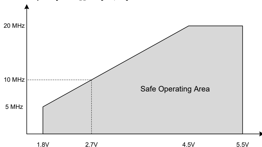
Figure 33-2. Maximum Frequency vs. V_{DD} for [85, 125]^{\circ}\text{C}
