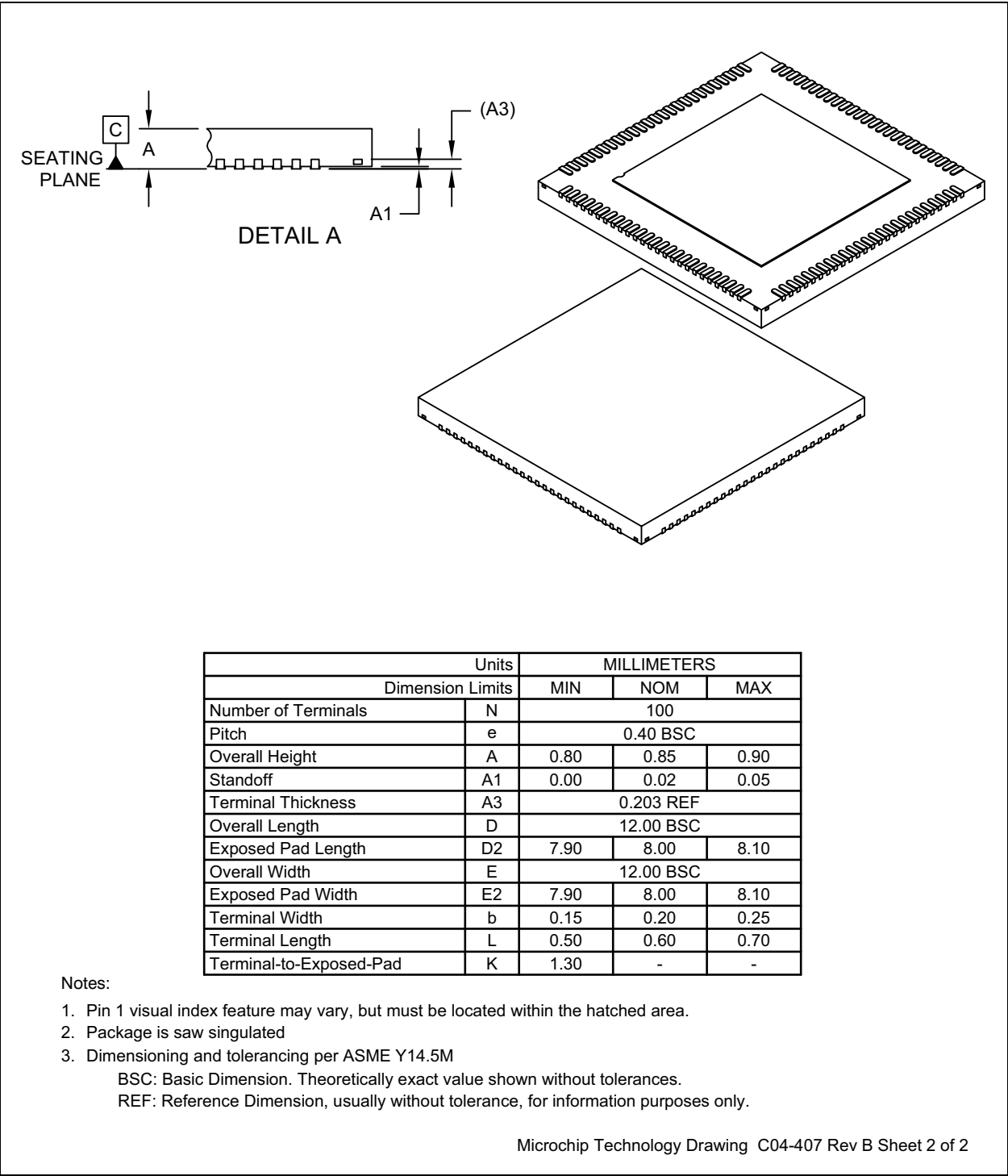
FIGURE 11-2: 100-VQFN PACKAGE (DIMENSIONS)
