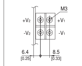
Terminal in detail (Module S, T, U)
