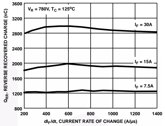
Figure 8. Reverse Recovered Charge vs di_F/dt
