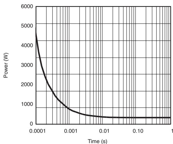
Single Pulse, Junction-to-Case ( T_C = 25\text{ }^{\circ}\text{C} )
