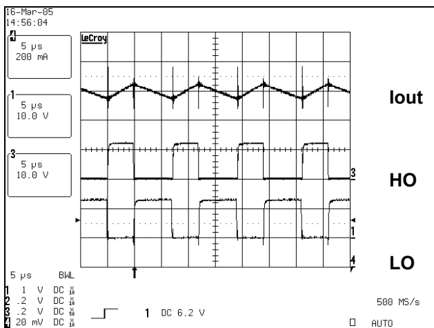
Fig.1 IRS254(01,11) Control Signals, lavg=1.2 A
