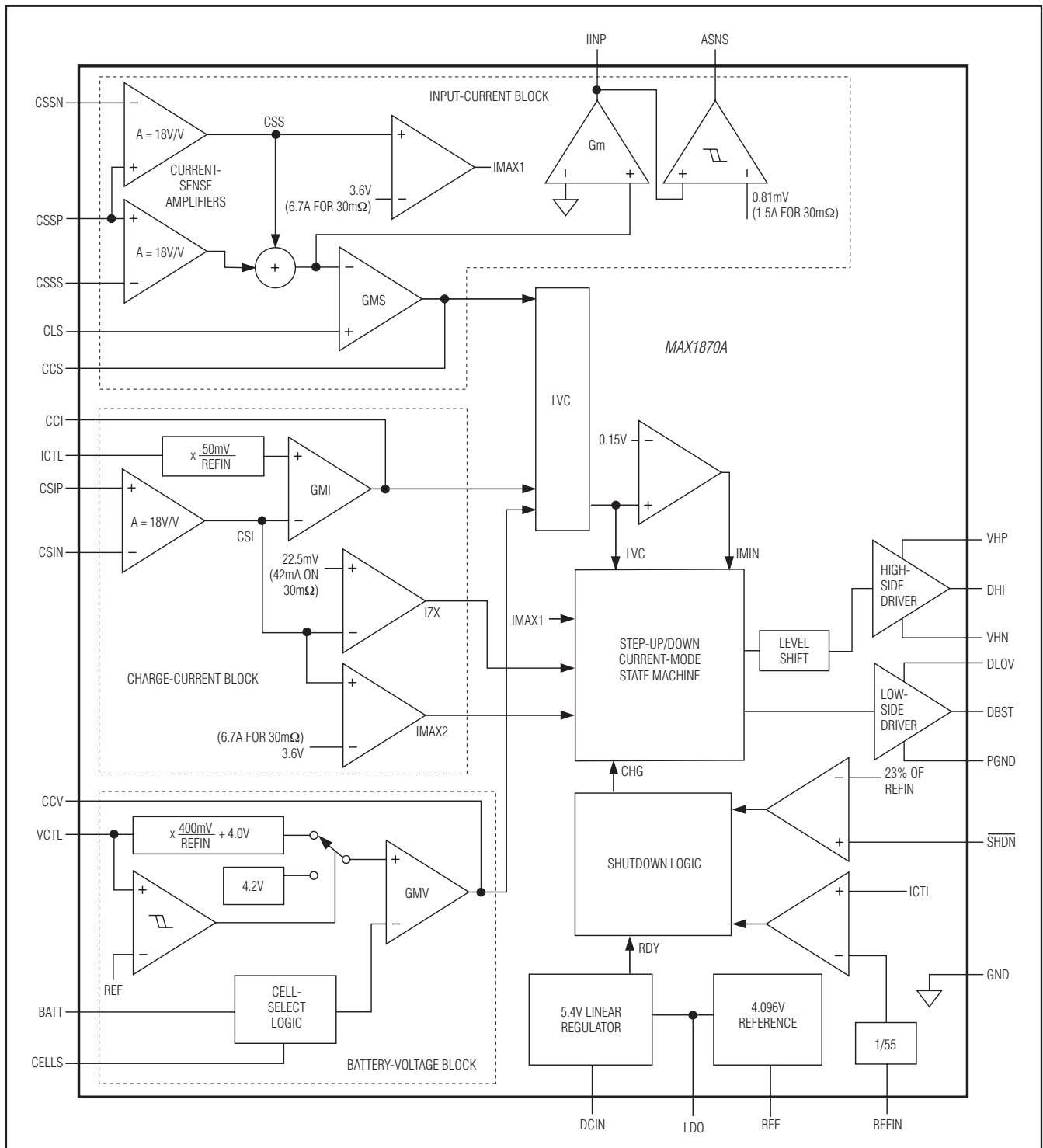
Figure 3. Functional Diagram
