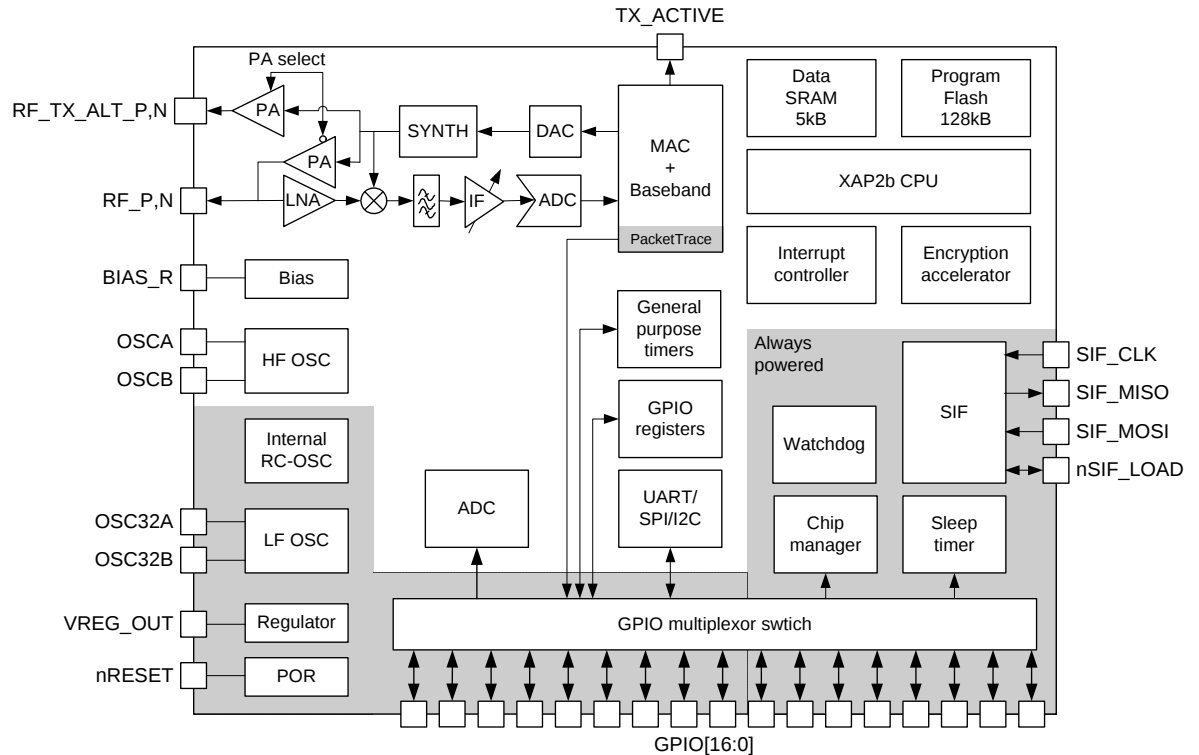
Figure 2. EM250 Block Diagram
