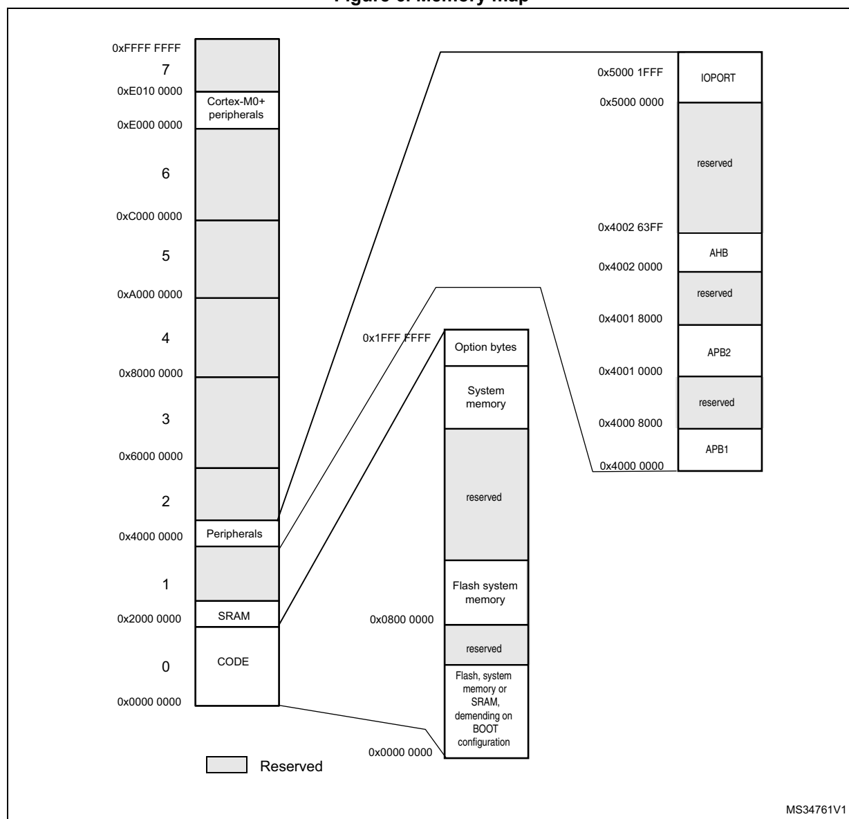
Figure 6. Memory map
