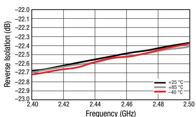
Figure 19. Small Signal Reverse Isolation (IS12) vs Frequency and Temperature, Narrow Band
