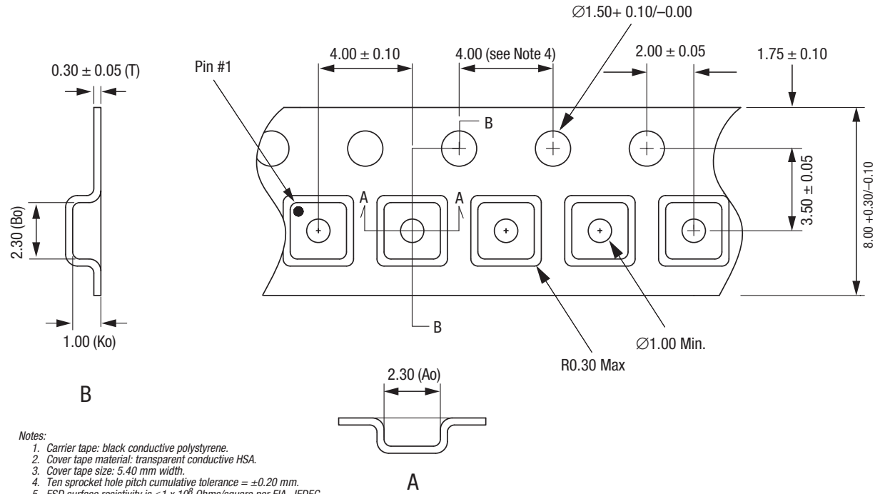
Figure 32. SKY67014-396LF Tape and Reel Dimensions
