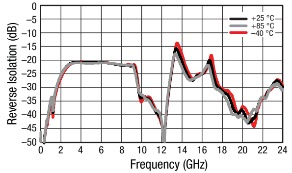
Figure 10. Small Signal Reverse Isolation (S12) vs Frequency and Temperature, Wide Band
