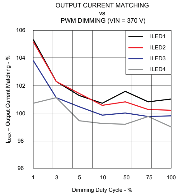
Figure 6. V_{IN} = 370 V, Current Matching
