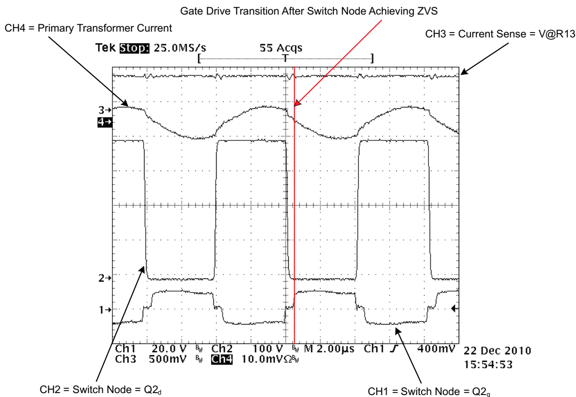
Figure 10. V_{IN} = 390 V, Outputs Loaded with 32, Cree XLamp CR-E , LEDs
