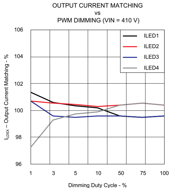
Figure 7. V_{IN} = 410 V, Current Matching
