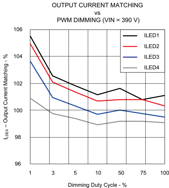
Figure 5. V_{IN} = 390 V, Current Matching
