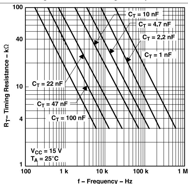
Figure 10. Timing Resistance vs Frequency
