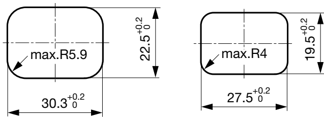
Rear panel mounting
