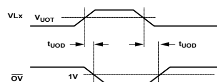
Figure 22. VLx Positive Voltage Monitoring Timing Diagrams
