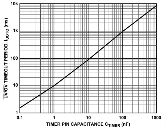
Figure 15. \overline{UV}/\overline{OV} Timeout Period vs. Capacitance
