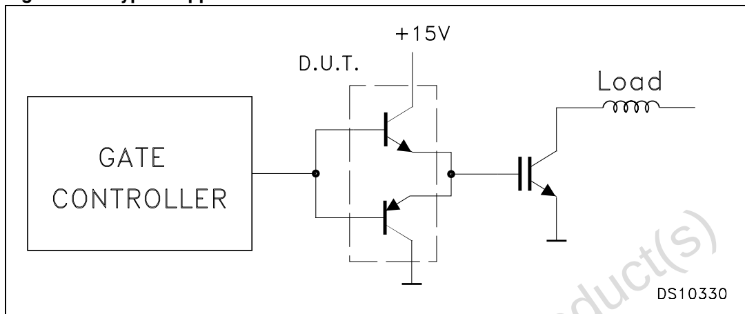
Figure 11. Typical application
