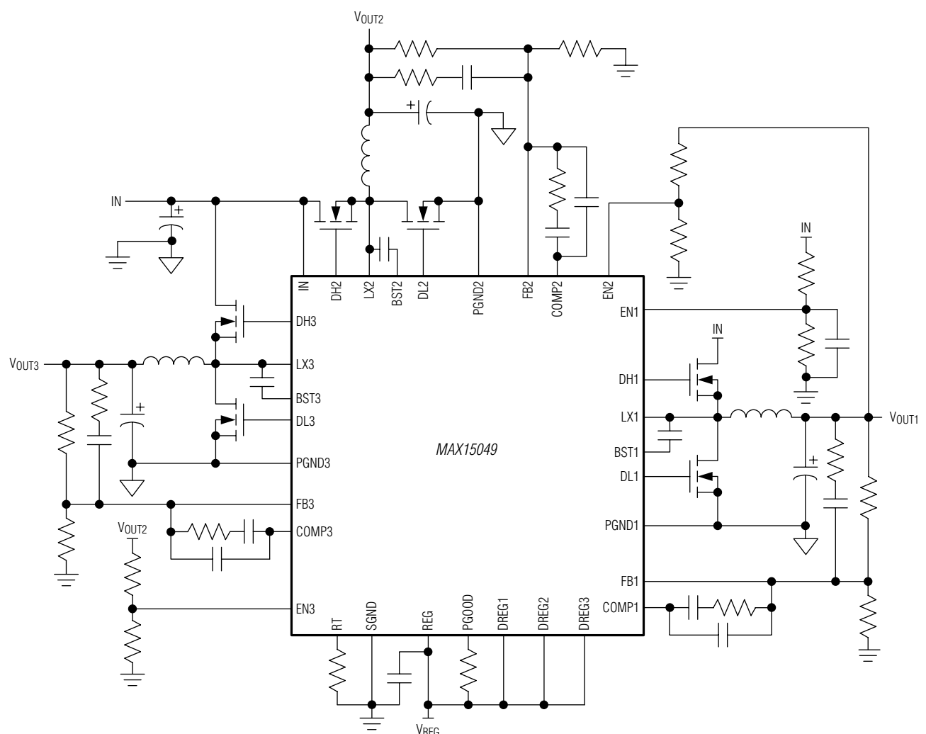
Figure 9. MAX15049 Sequencer Typical Operating Circuit
