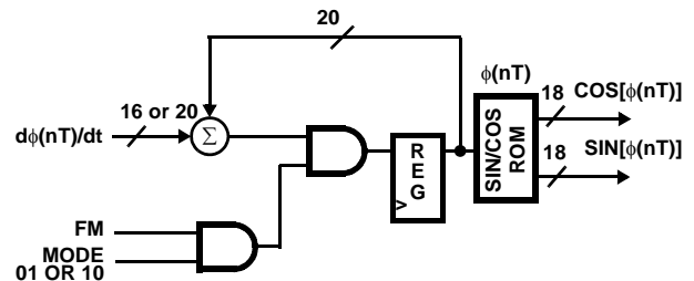
FIGURE 10. FM MODULATOR BLOCK DIAGRAM
