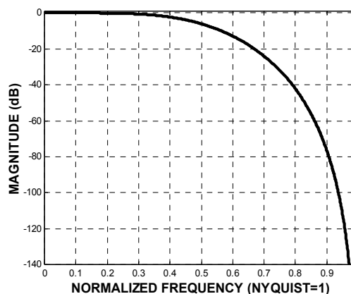
FIGURE 12. HALF BAND FILTER RESPONSE
