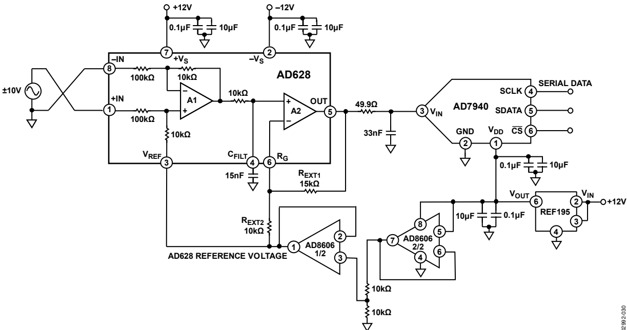
Figure 32. Level Shifter
