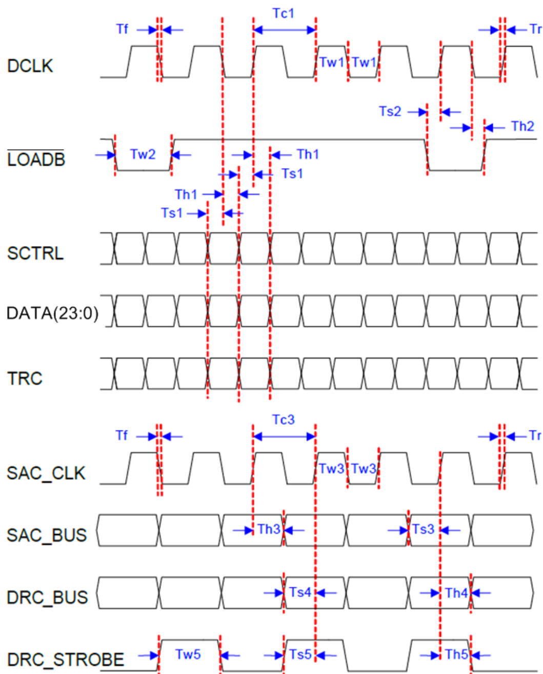
Figure 13. Switching Characteristics
