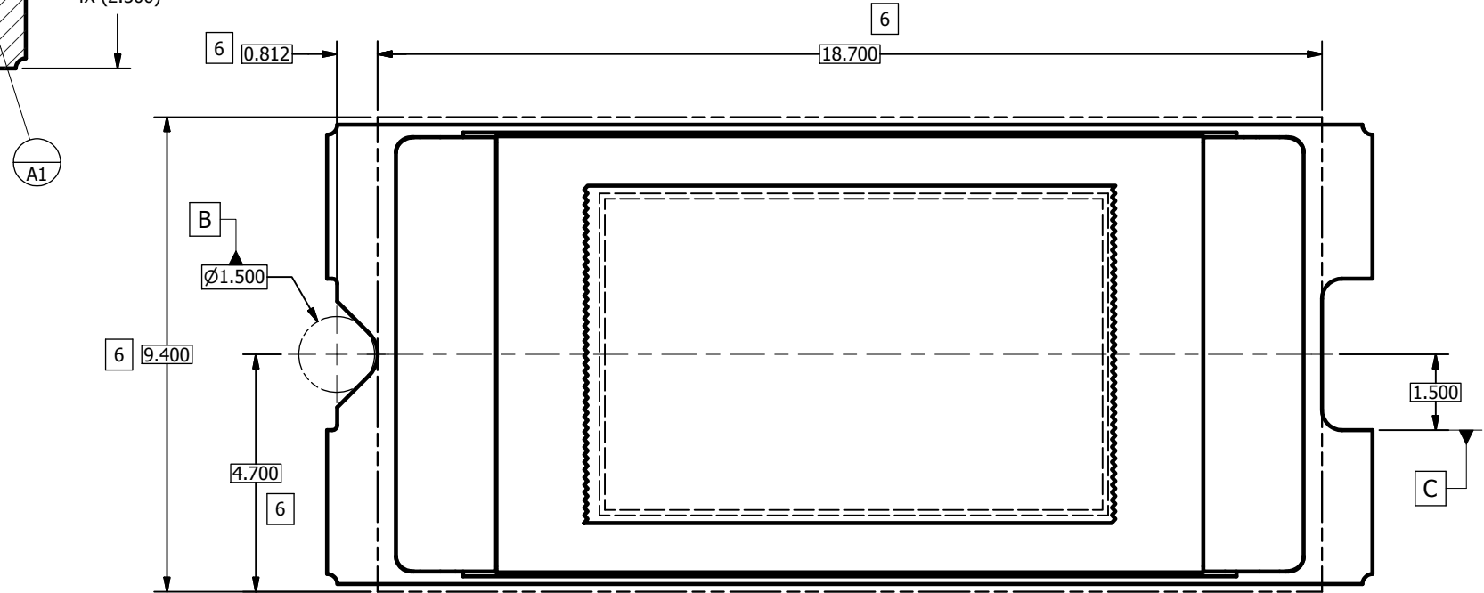
VIEW C ENCAPSULANT MAXIMUM X/Y DIMENSIONS SCALE 15 : 1 (FROM SHEET 1)
