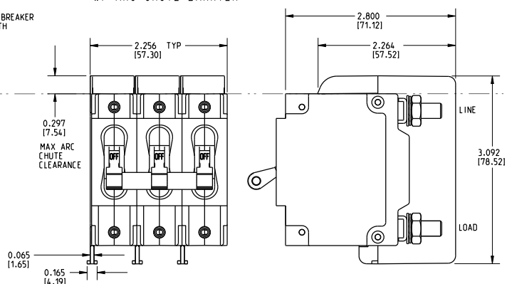
3-POLE (CA3) w/ ARC CHUTE BARRIER
