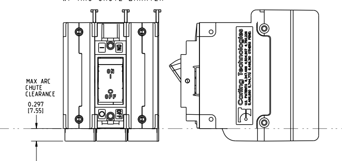
3-POLE (CF3,CG3,C13,C23) w/ ARC CHUTE BARRIER
