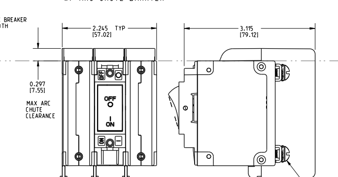
3-POLE (CC3,CD3) w/ ARC CHUTE BARRIER
