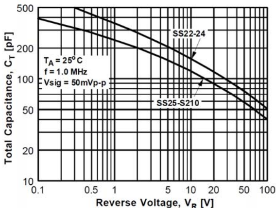
Figure 4. Total Capacitance
