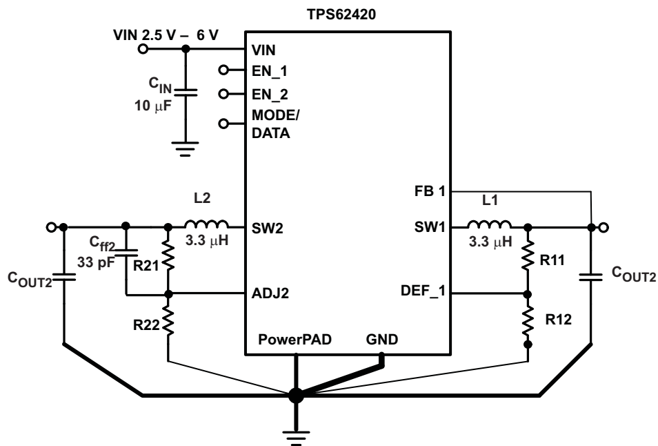
Figure 36. Layout Diagram
