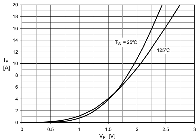
Fig. 21. Forward Current I_F vs V_F
