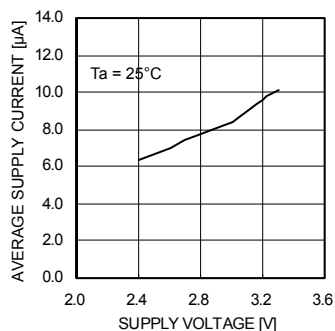
Fig.11 I DD - Supply voltage
