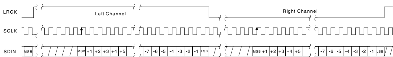
Figure 4. Right-Justified Data
