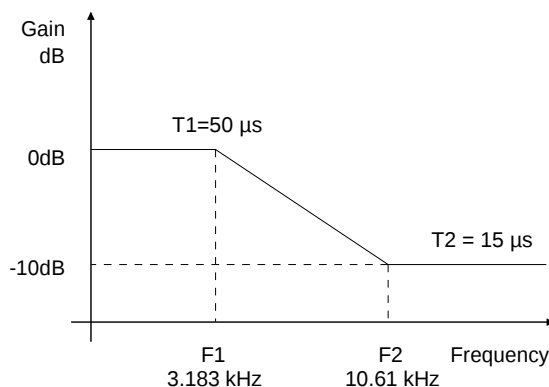
Figure 6. De-Emphasis Curve
