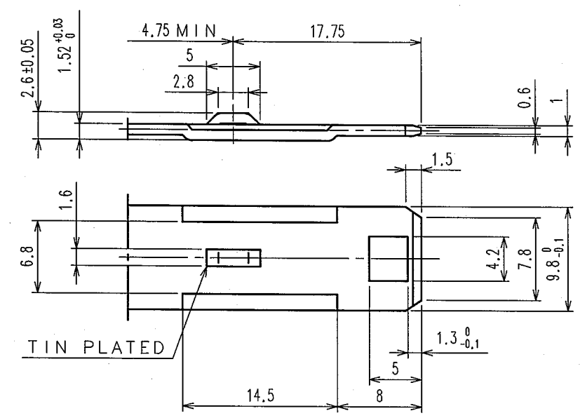
DETAIL OF FITTING PLATE(2:1)
