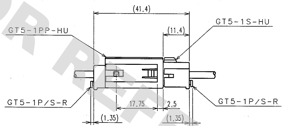
MATED CONNECTORS
