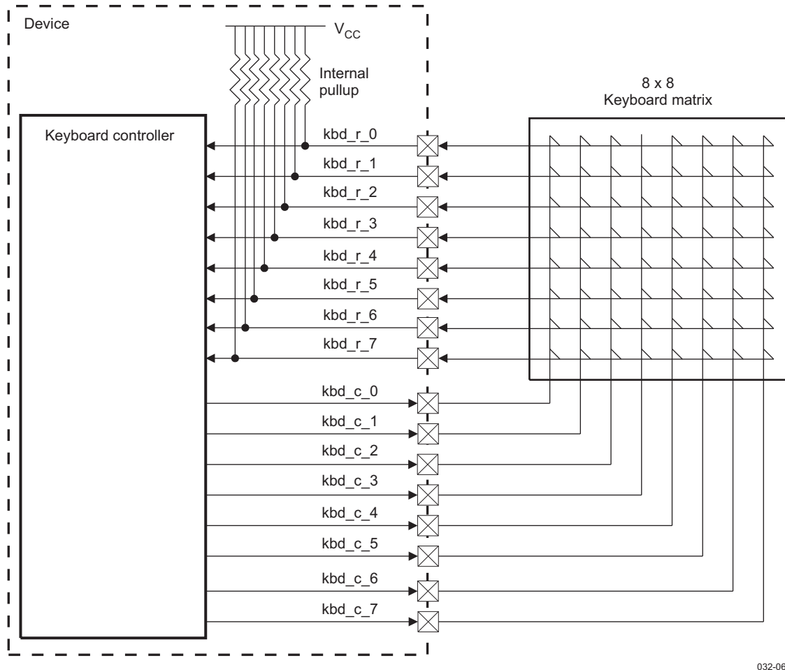
Figure 5-60. Keyboard Connection
