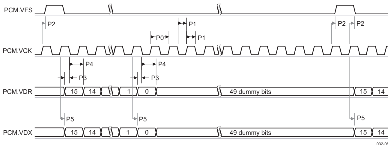
Figure 4-5. Voice/BT PCM Interface—Master Mode (Mode 1)
