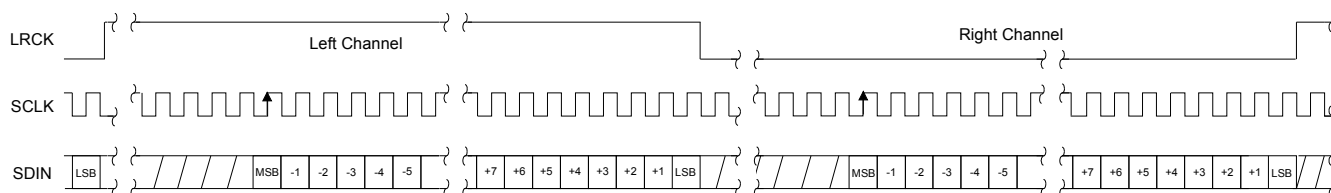
Figure 13. Right-Justified Data
