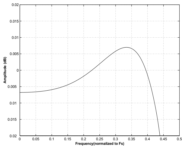
Figure 26. Single-Speed (slow) Passband Detail
