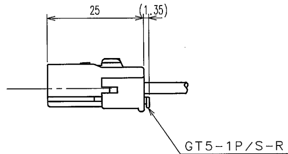
CONNECTOR ASSEMBLED WITH A RETAINER
