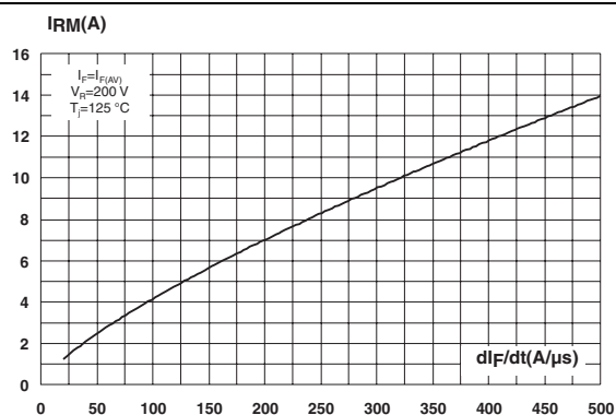
Figure 4. Peak reverse recovery current versus dl_F/dt (typical values, per diode)
