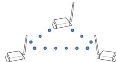
Figure 2-06. NonBeacon Peer-to-Peer Architecture
