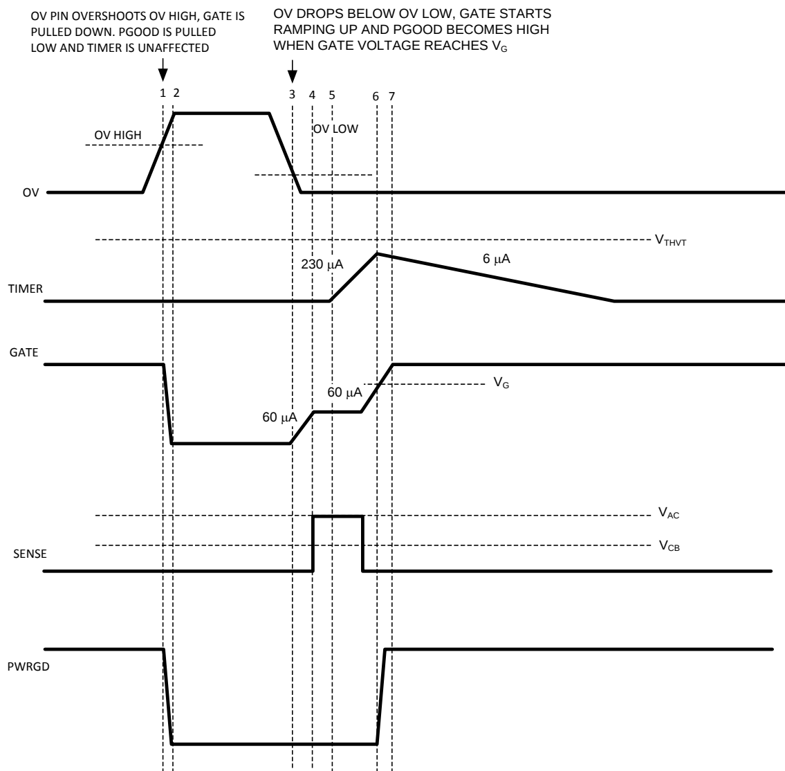
Figure 29. Over-Voltage Timing Behavior
