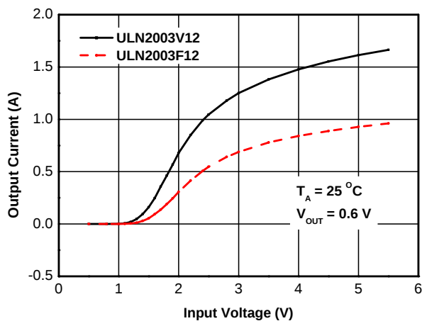
Output Current vs. Input Voltage (All Darlington's in Parallel)
