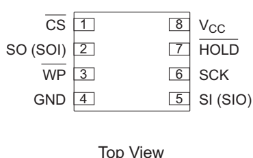
Figure 2-2. 8-pad UDFN
