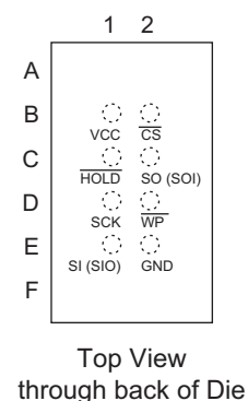
Figure 2-3. 8-ball dBGAs (WLSCP)
