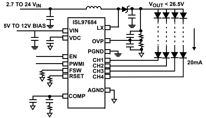
FIGURE 27. DUAL SUPPLIES 2.7V OPERATION
