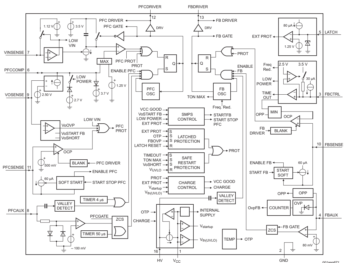
Fig 1. Block diagram
