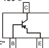
Pin Configuration Top View
