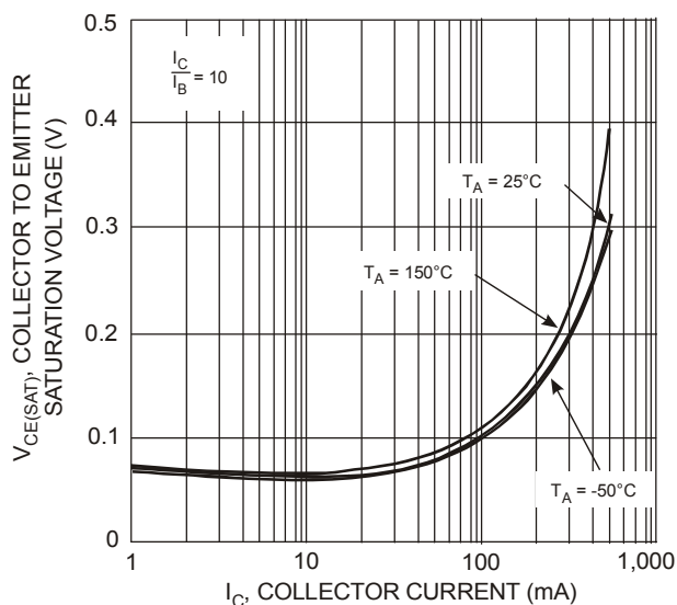
Fig. 4 Collector Emitter Saturation Voltage vs. Collector Current (4401)
