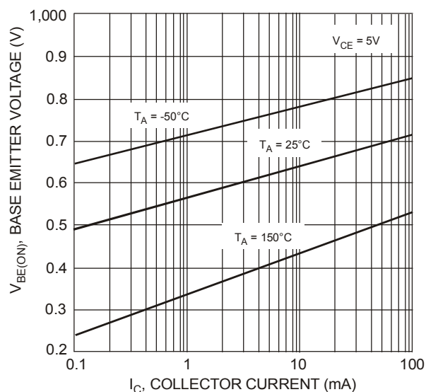
Fig. 10 Base-Emitter Voltage vs. Collector Current (4403)
