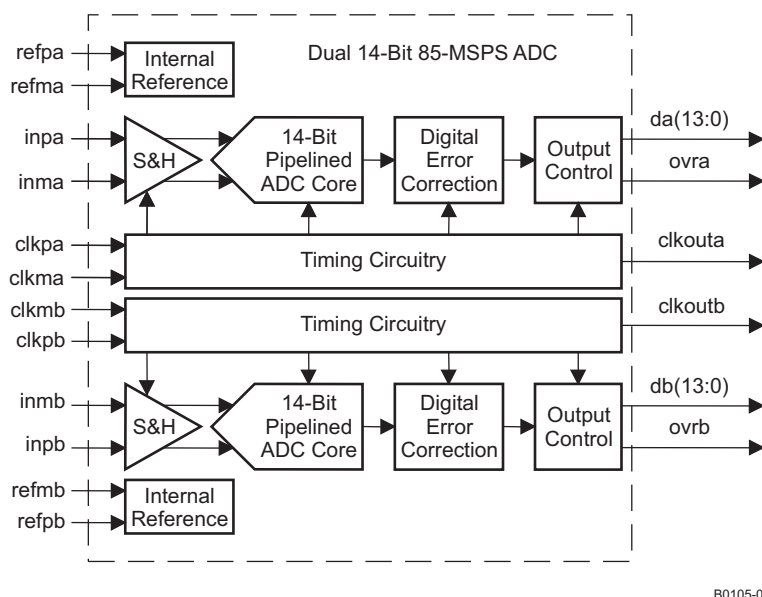
Figure 6-1. ADC Block Diagram
