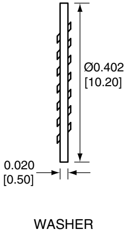
WASHER
