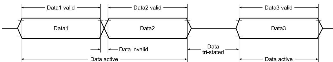
Figure 9. Signal states
