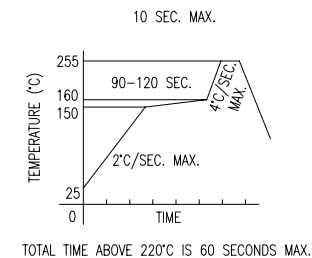
LEAD FREE REFLOW PROFILE
