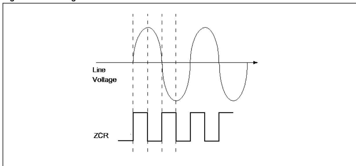
Figure 15. ZCR signal
