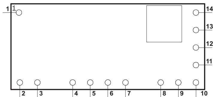
PTH08T210W (TOP VIEW)
