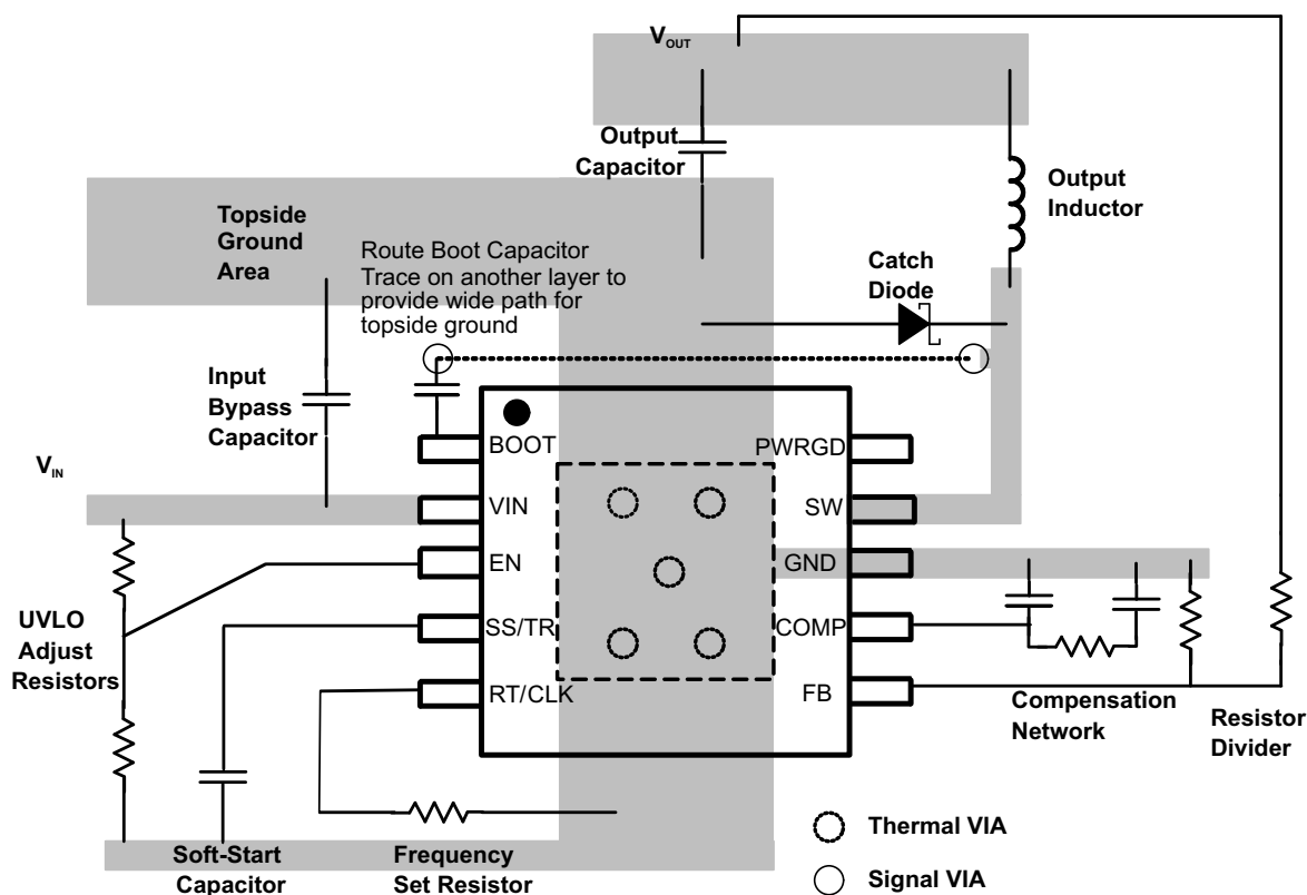
Figure 71. PCB Layout Example
