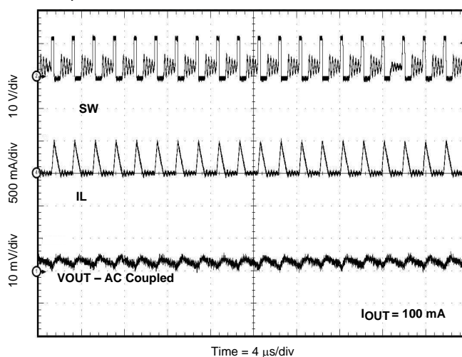
Figure 52. Output Ripple DCM
