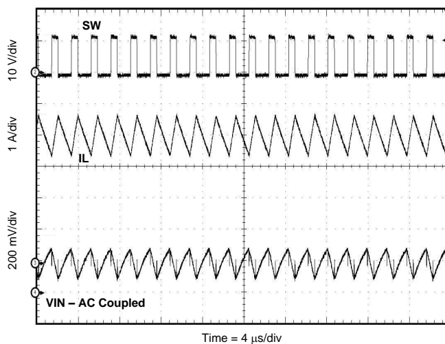
Figure 54. Input Ripple CCM
