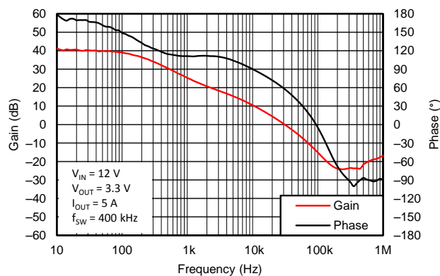
Figure 64. Overall Loop Frequency Response
