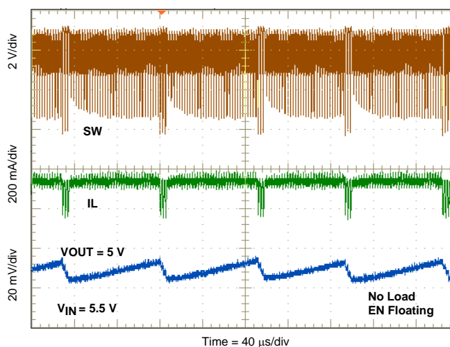
Figure 56. Low Dropout Operation
