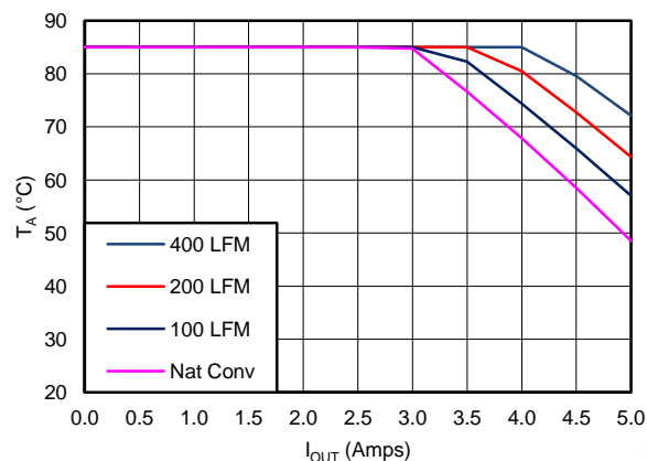
Figure 70. Air Flow Conditions V_{IN} = 36 V, V_O = 12 V
