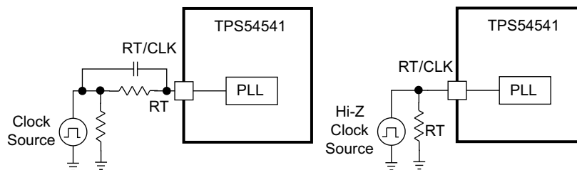
Figure 38. Synchronizing to a System Clock
