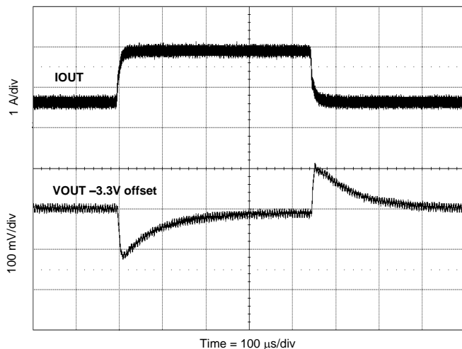
Figure 47. Load Transient
