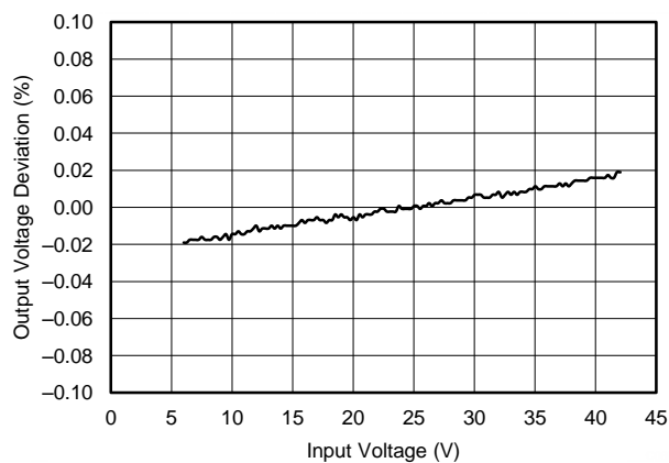
Figure 66. Regulation vs Input Voltage
