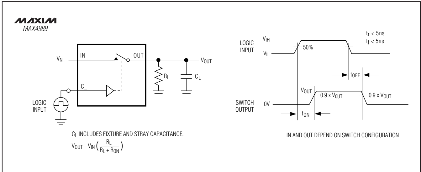
Figure 2. Switching Time
