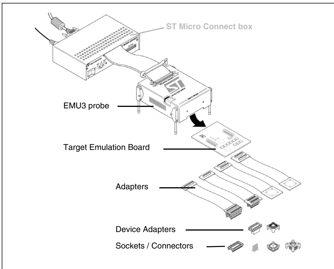
Figure 1: ST7MDTxxx-EMU3 terminology
