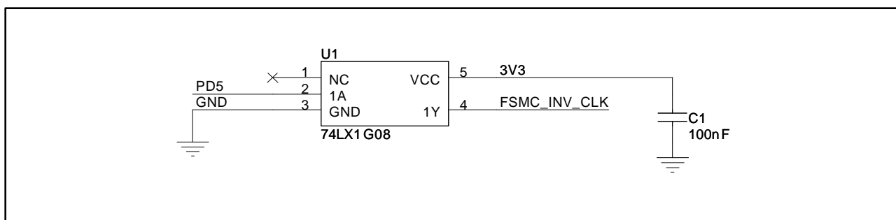
Figure 2: Single channel inverter
